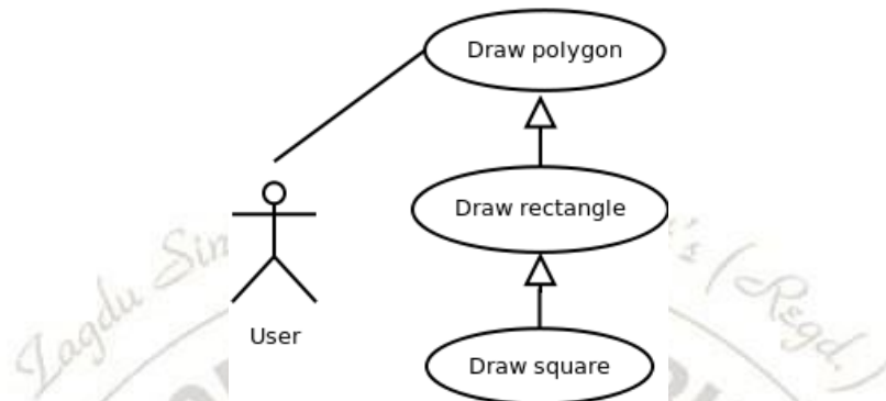
Figure - 04: Generalization relationship among use cases
