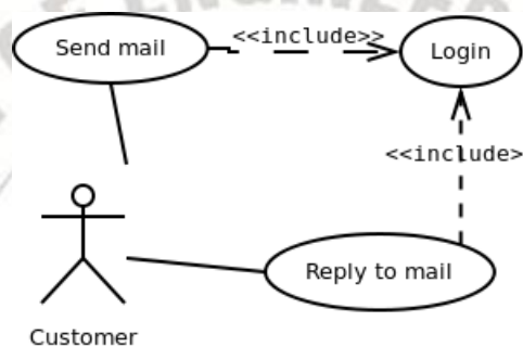
Figure - 02: Include relationship between use cases
